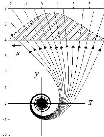
Fig. 8. The figure shows several field lines for a dipole that rotates counterclockwise in the xy plane. The image plane here is located at q_0 = 4 , and at \theta_0 = \phi_0 = \pi/2 , so perpendicular to the y axis. The field line in the (\theta_0, \phi_0) direction intersects the image plane at \bar{x} = 2 and the maximum of the intensity profile is located at \bar{x} = 2/3 .
